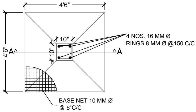
PLAN OF COLUMN FOUNDATION SCALE= 1:50
