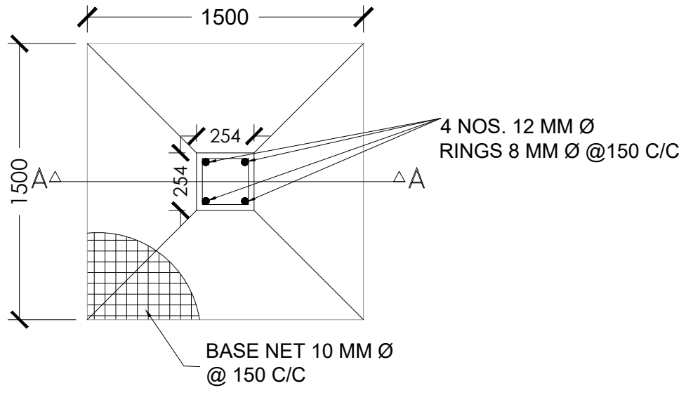
PLAN OF COLUMN FOUNDATION
