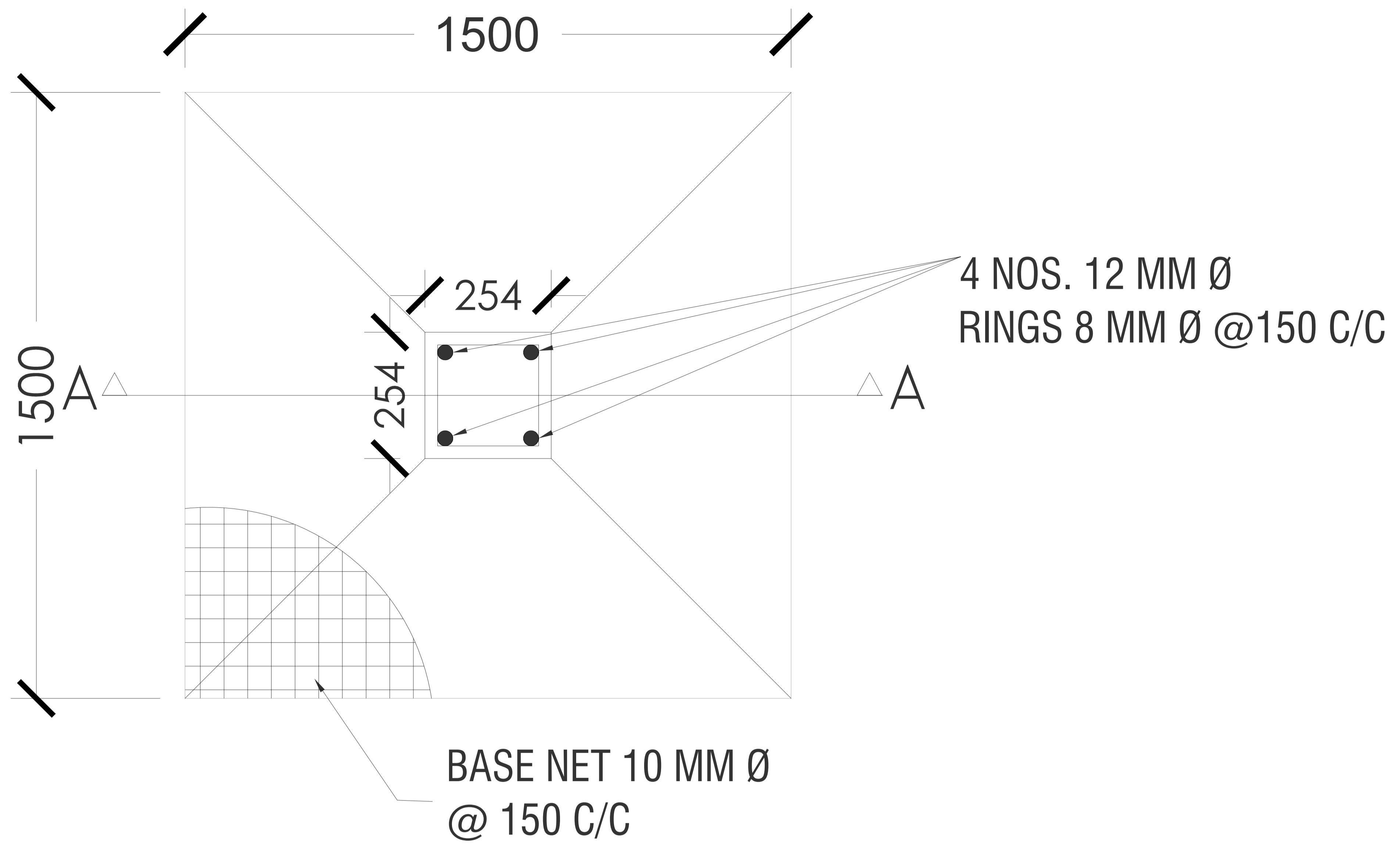
PLAN OF COLUMN FOUNDATION
