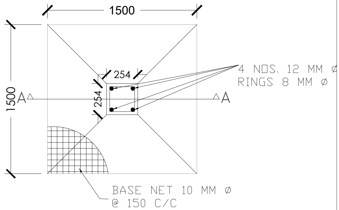
PLAN OF COLUMN FOUNDATION
