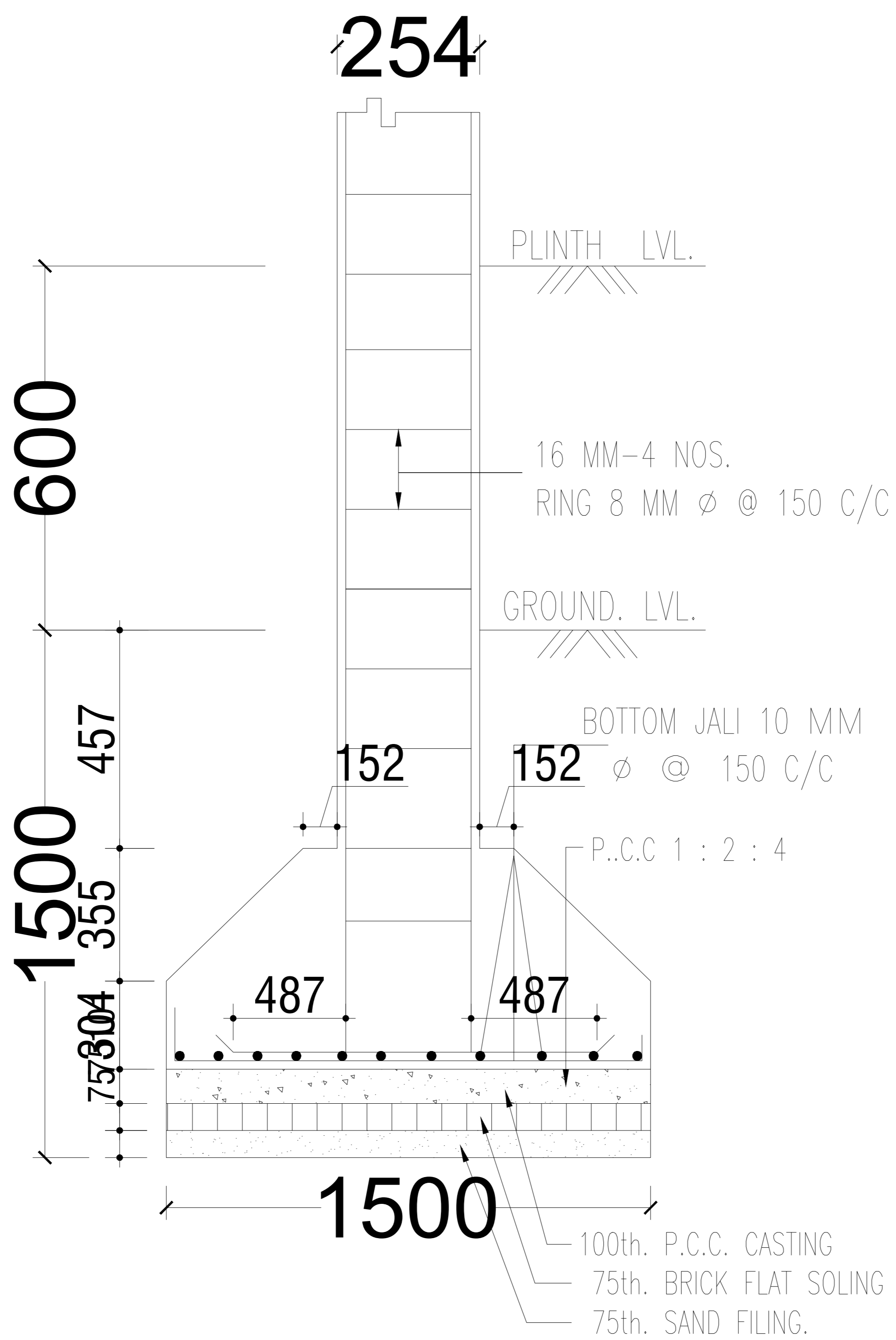
SECTION ON A-A
