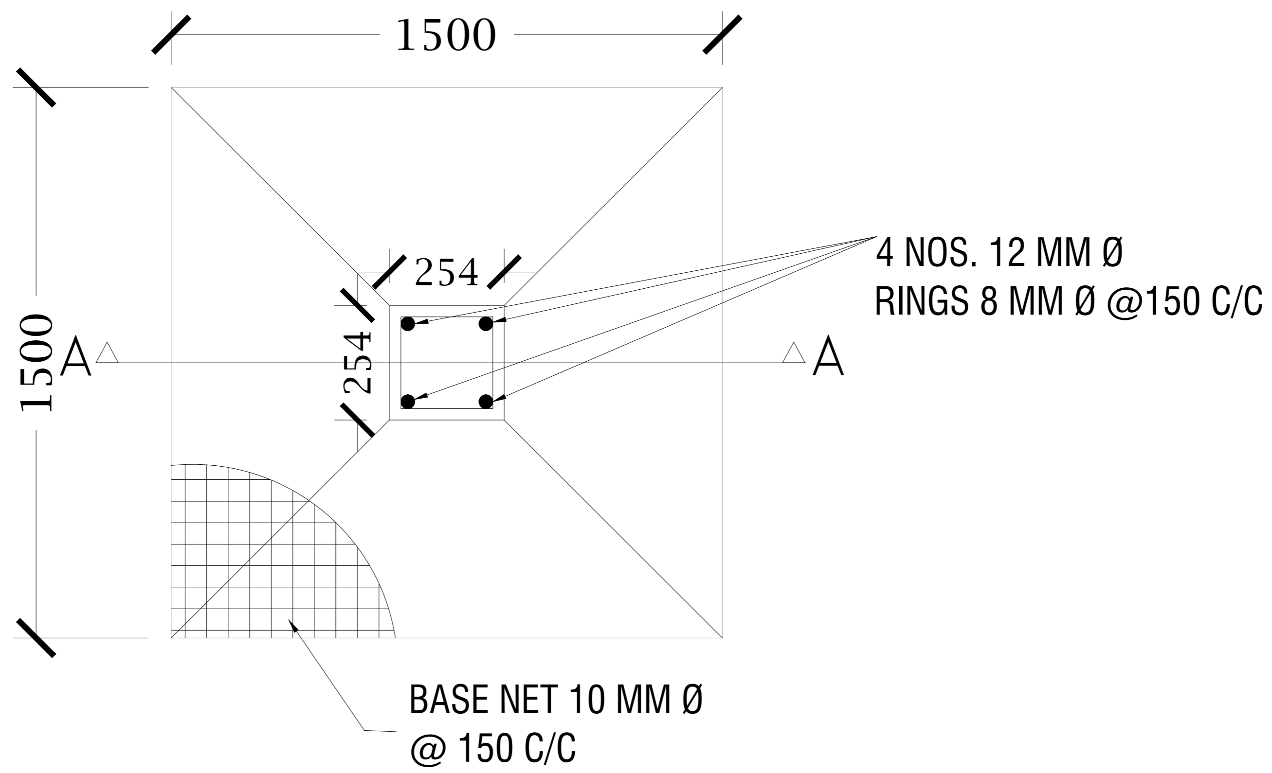
PLAN OF COLUMN FOUNDATION
