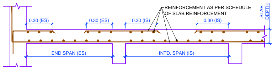
TYPICAL REINFORCEMENT OF SLAB
