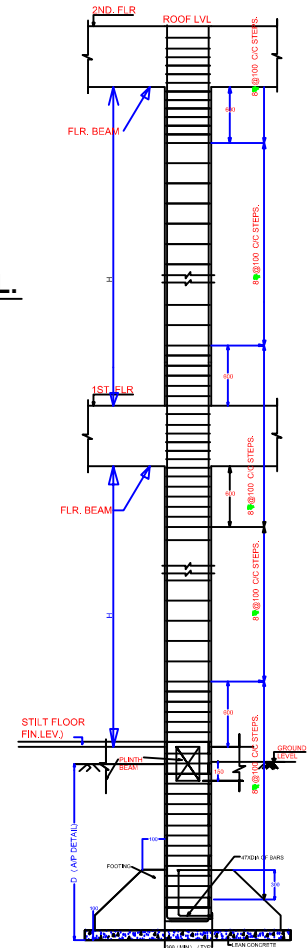
TYPICAL DETAIL OF COLUMN SHOWING COLUMN TIES
