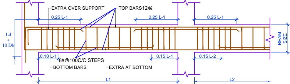
TYPICAL DETAILS OF BEAMS REINFORCEMENT
