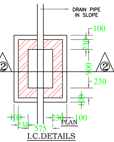
I.C. DETAILS
