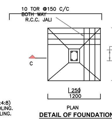
DETAIL OF FOUNDATION
