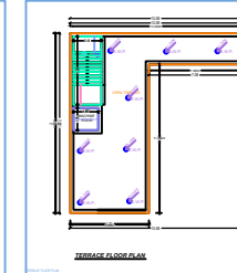
TERRACE FLOOR PLAN
