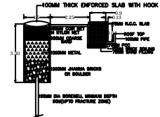
DETAIL OF RECHARGE WELL
