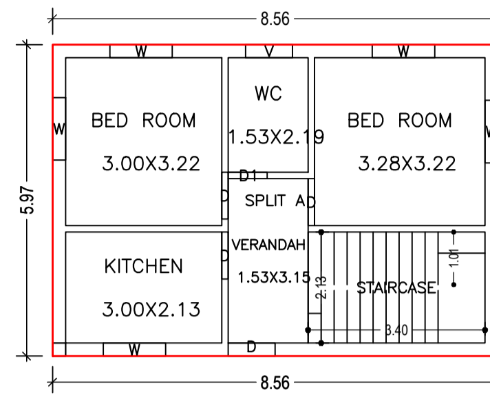
FIRST FLOOR PLAN (Proposed) (SCALE 1:100)
