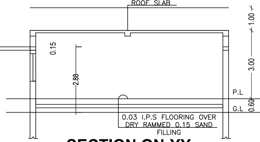
SECTION ON-YY
