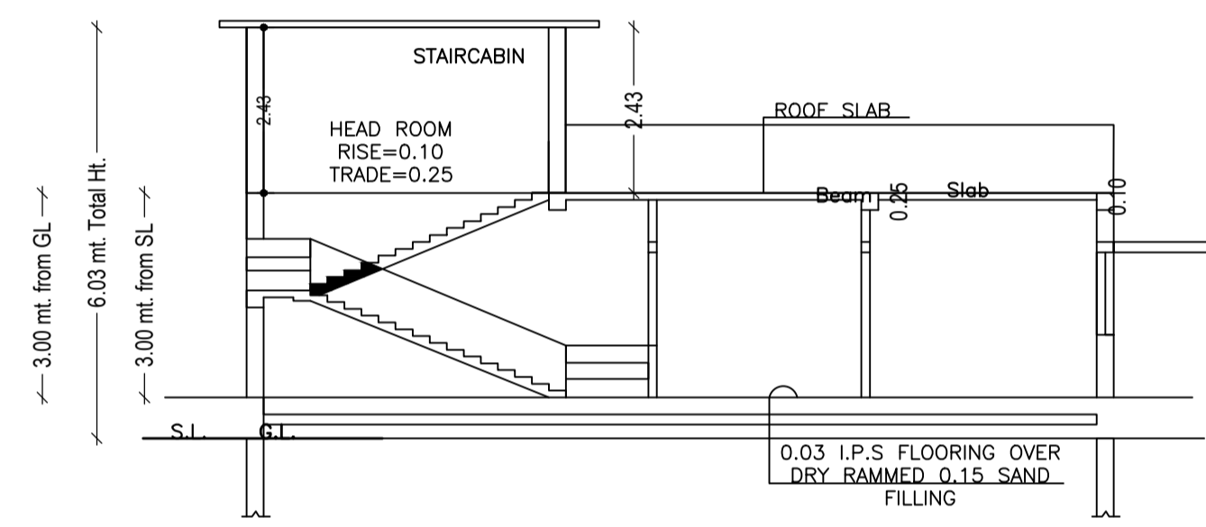
SECTION ON-XX
