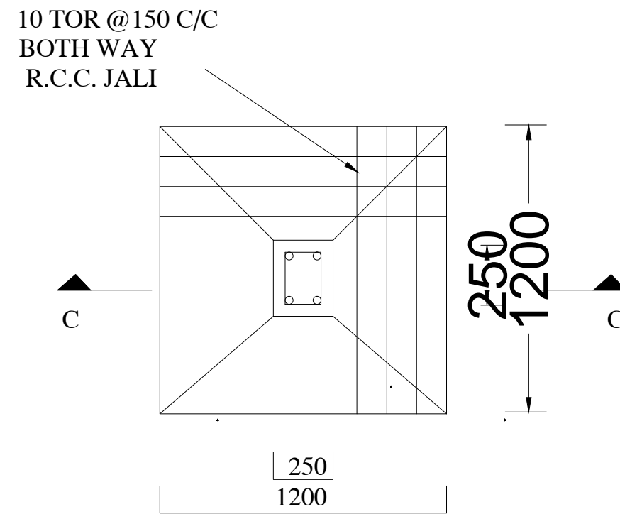
PLAN DETAIL OF FOUNDATION
