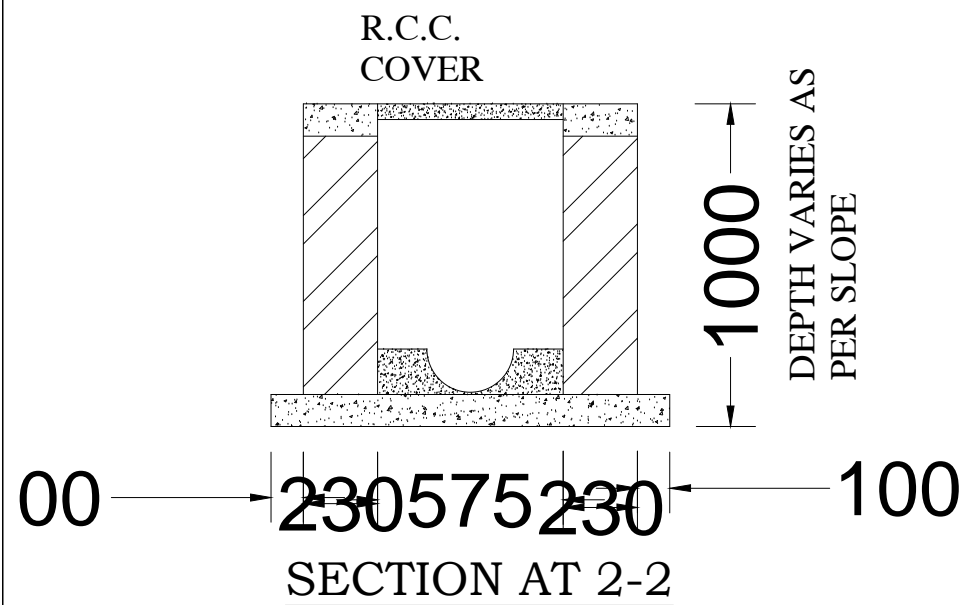
STRUCTURE DETAIL
