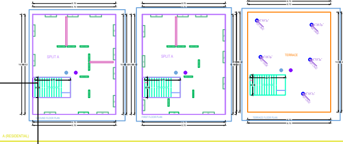
Building A (RESIDENTIAL)
