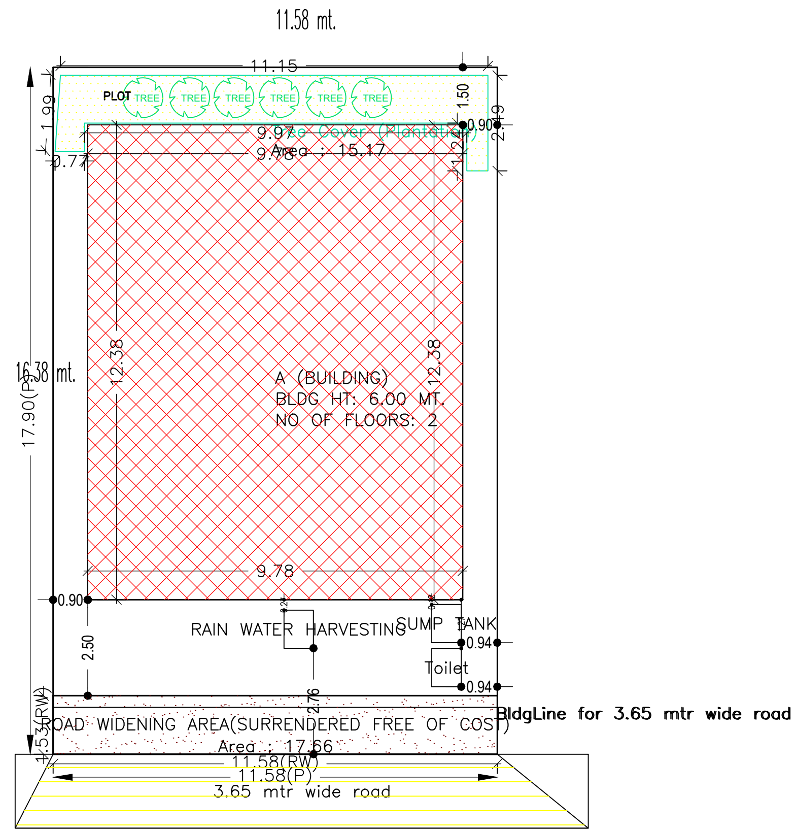
site plan
