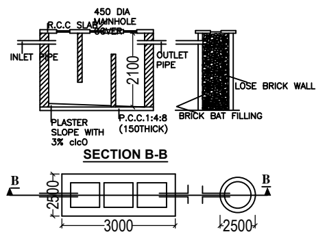
DETAIL OF SEPTIC TANK & SOAKPIT SCALE - 1:50
