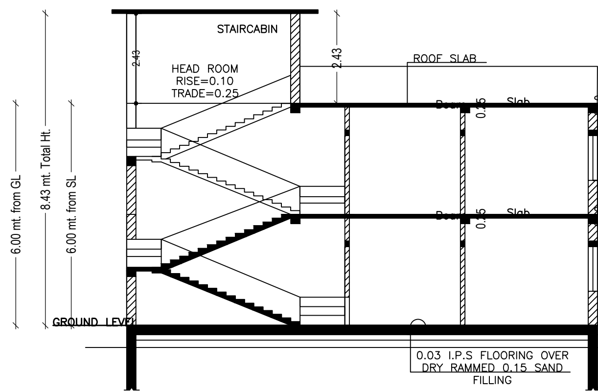
SECTION ON-XX
