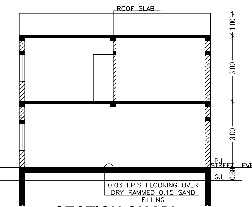
SECTION ON-YY
