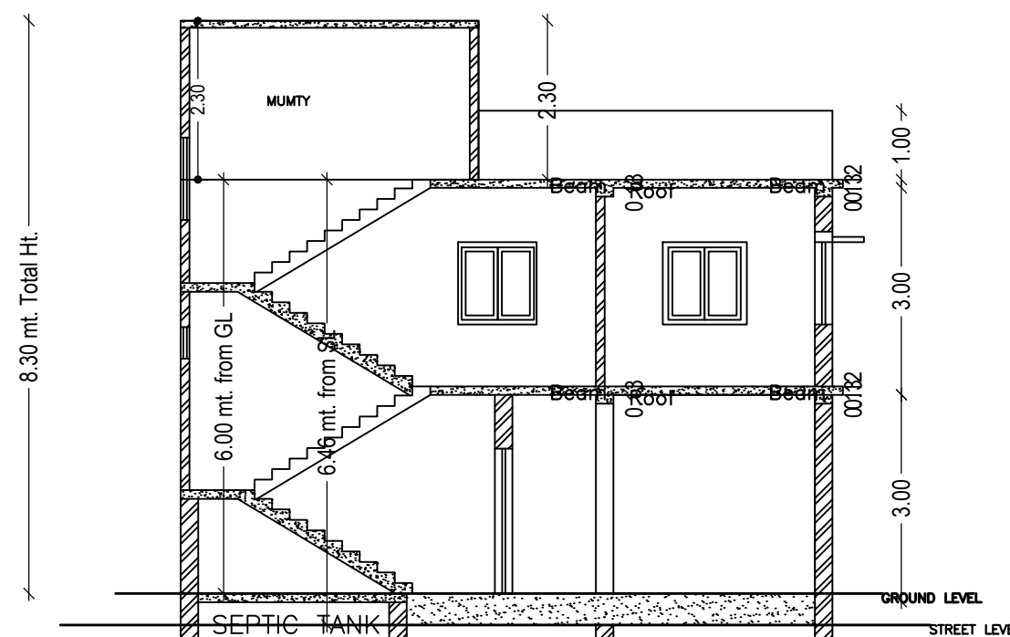
SECTION DETAILS (SCALE 1:100)
