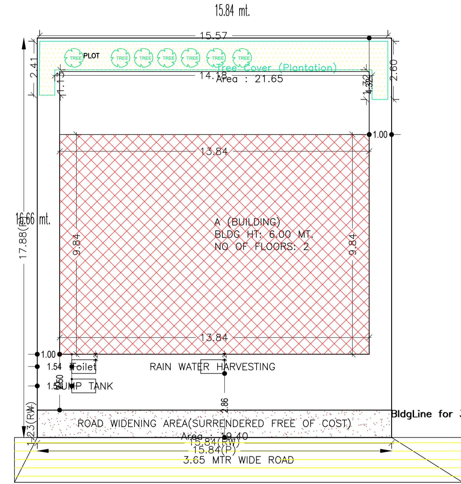
SITE PLAN
