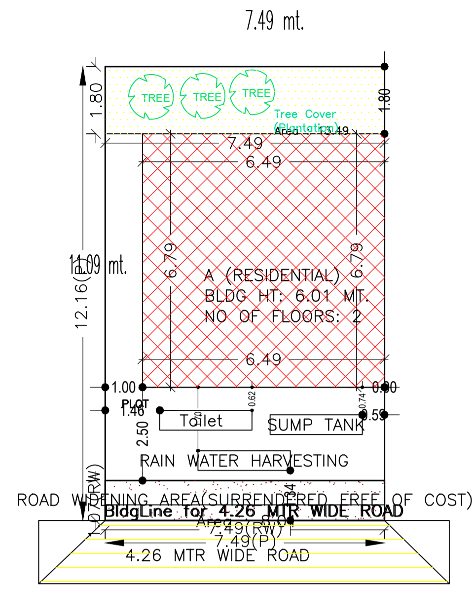
SITE PLAN
