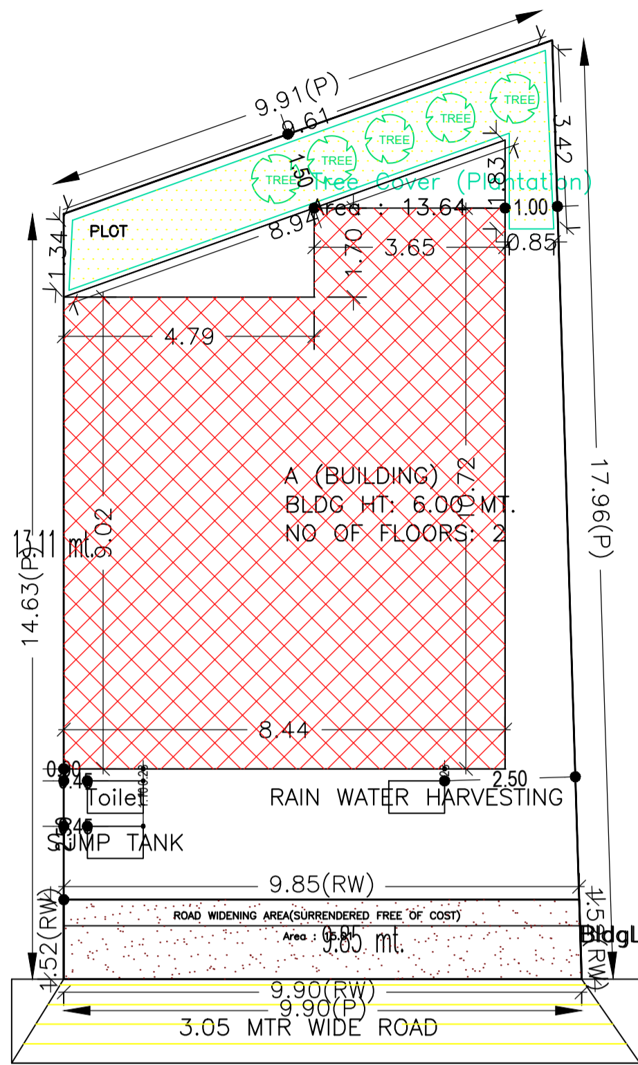
SITE PLAN
