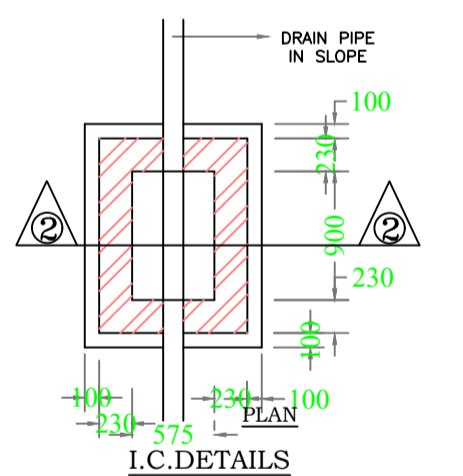
I.C. DETAILS
