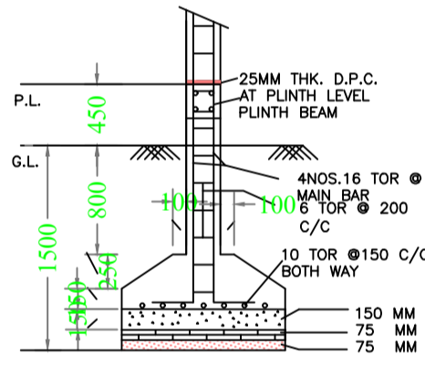
STRUCTURAL DETAIL
