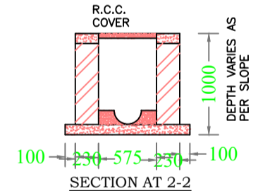
SECTION AT 2-2
