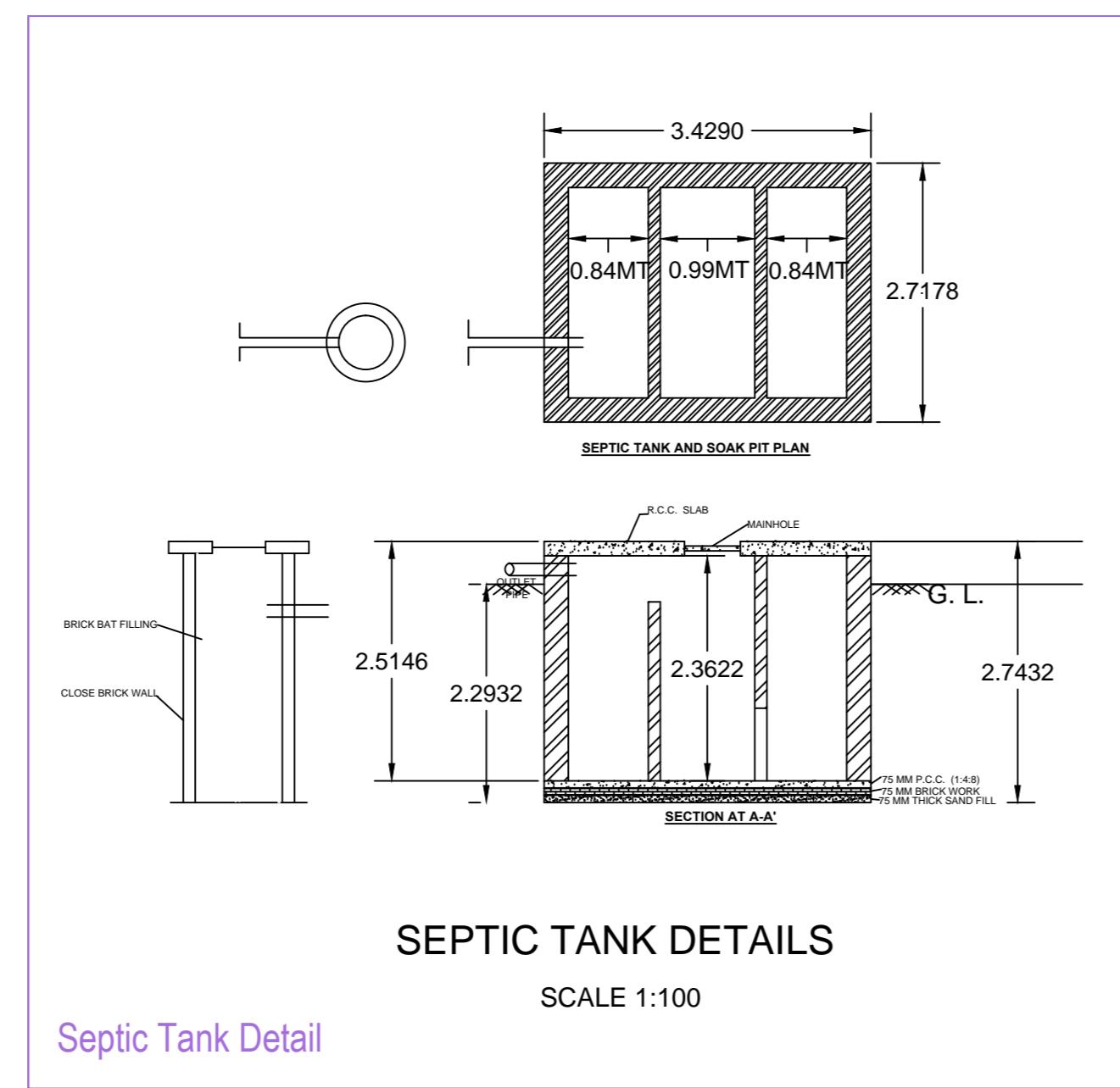
Structure Detail
