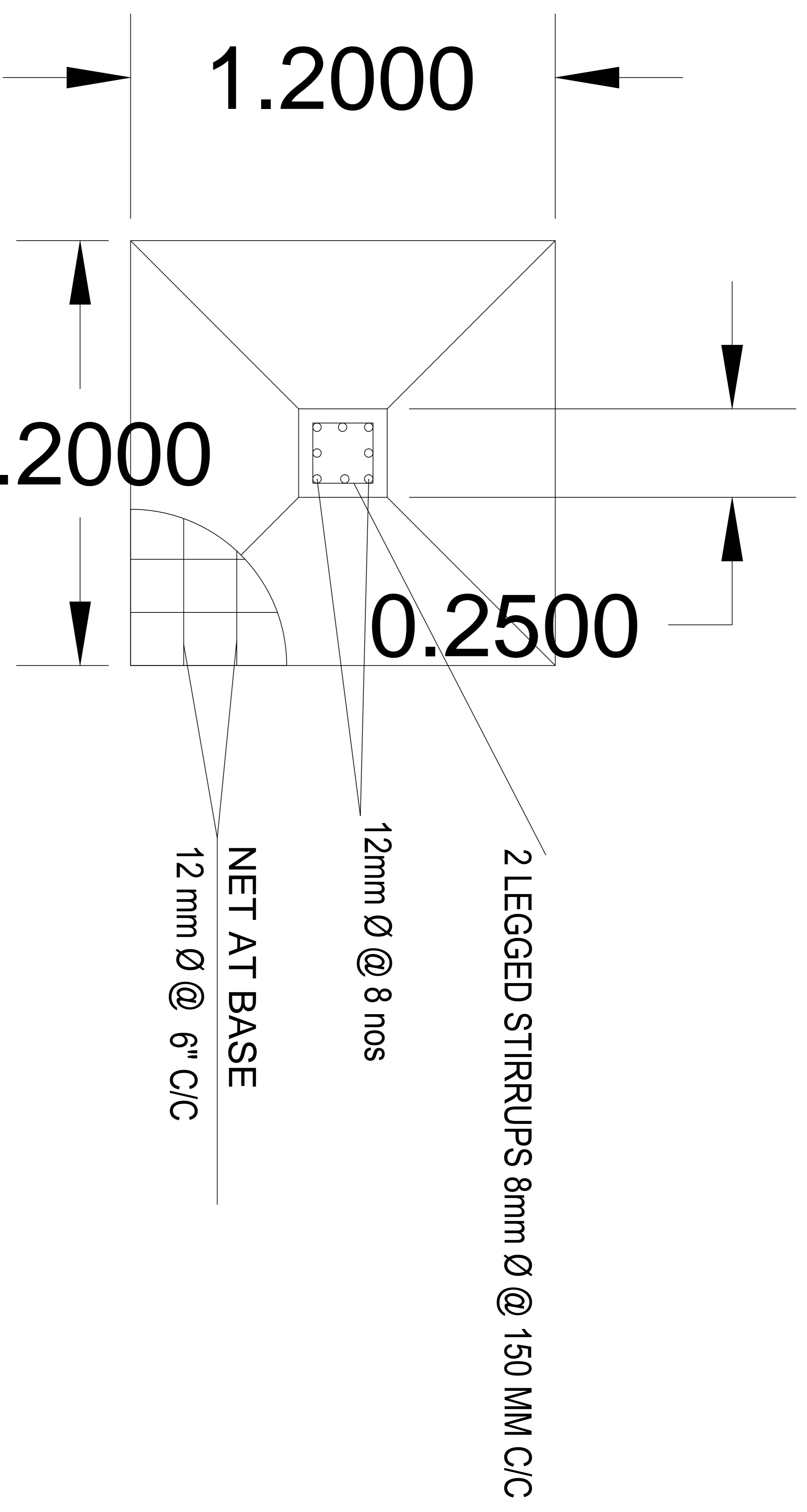
PLAN OF COLUMN FOUNDATION
