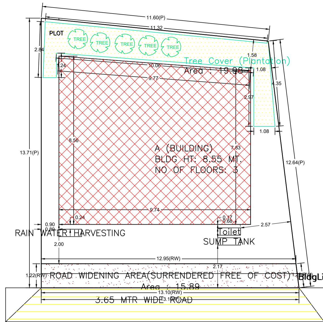
SITE PLAN
