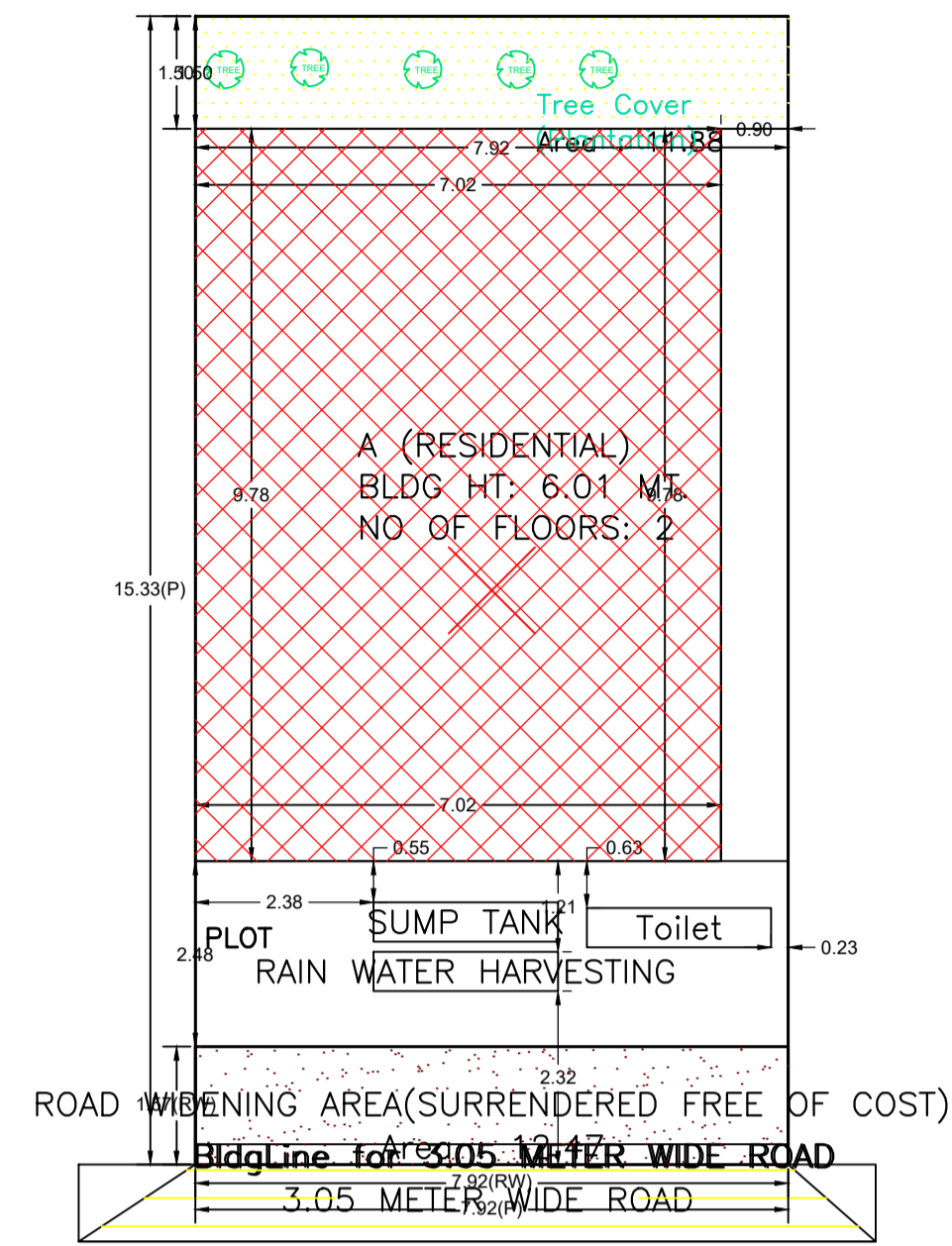
SITE PLAN
