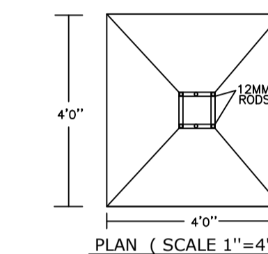
PLAN ( SCALE 1"=4' )
