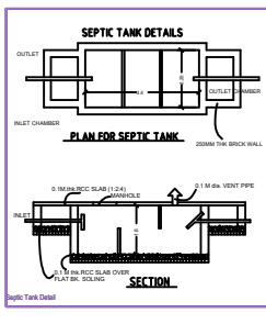
SEPTIC TANK DETAILS PLAN FOR SEPTIC TANK SECTION
