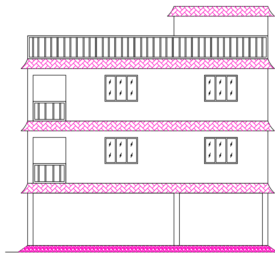
FRONT ELEVATION
