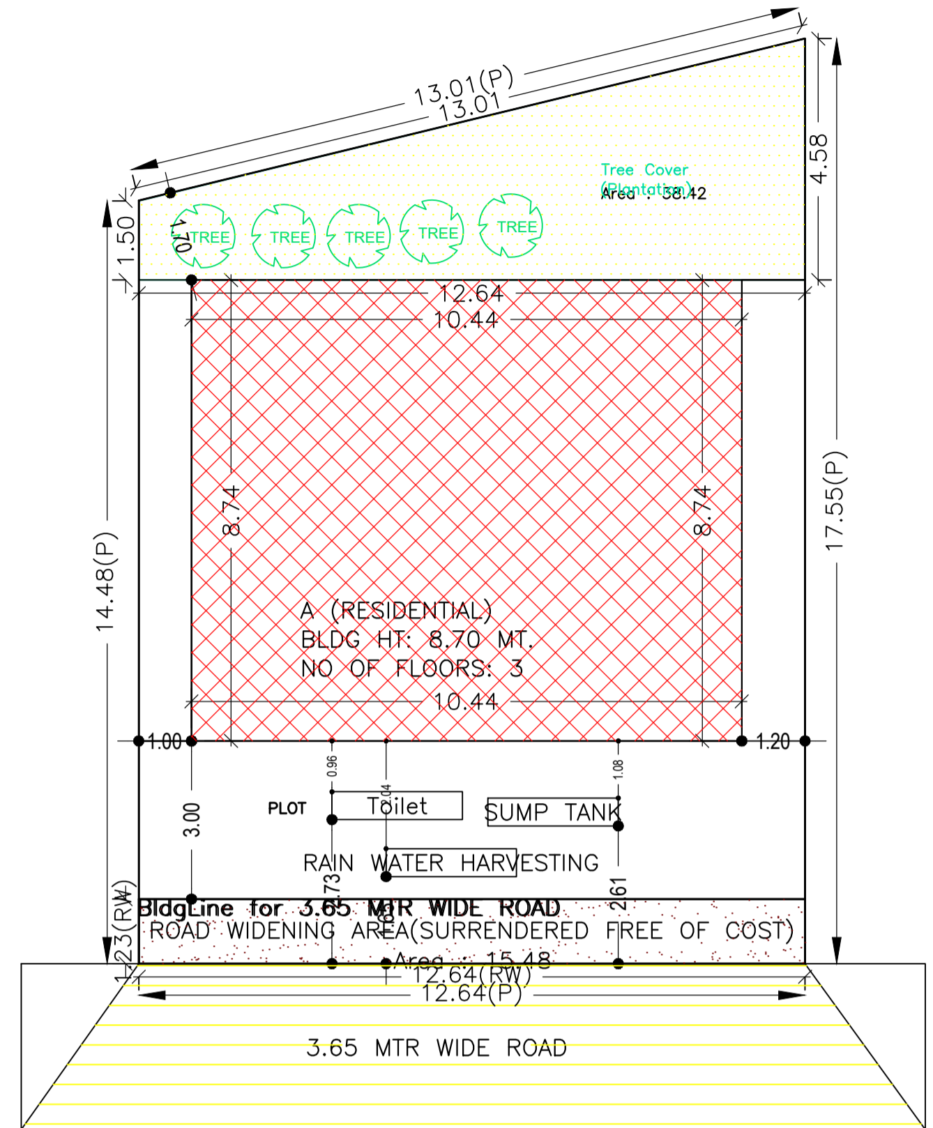
SITE PLAN
