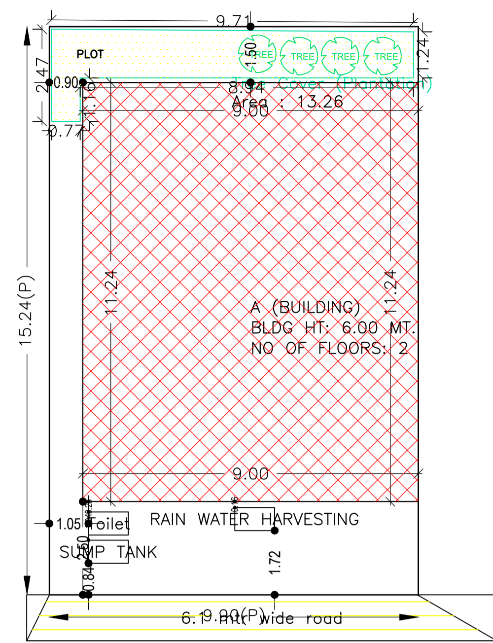
SITE PLAN
