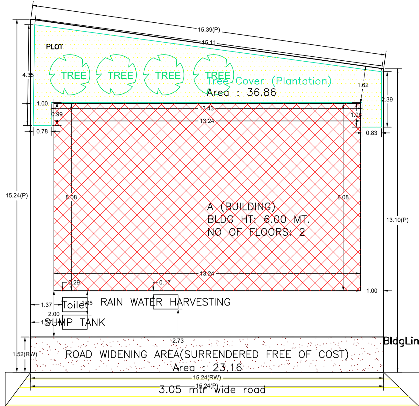
SITE PLAN
