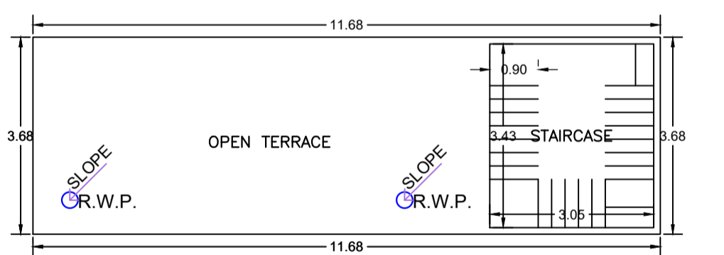
TERRACE FLOOR PLAN (Proposed) (SCALE 1:100)
