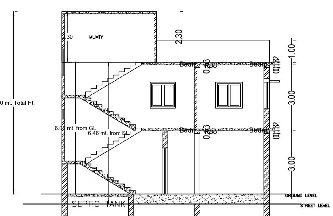
SECTION DETAILS (SCALE 1:100)
