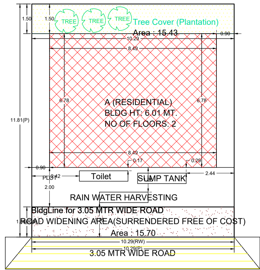
SITE PLAN
