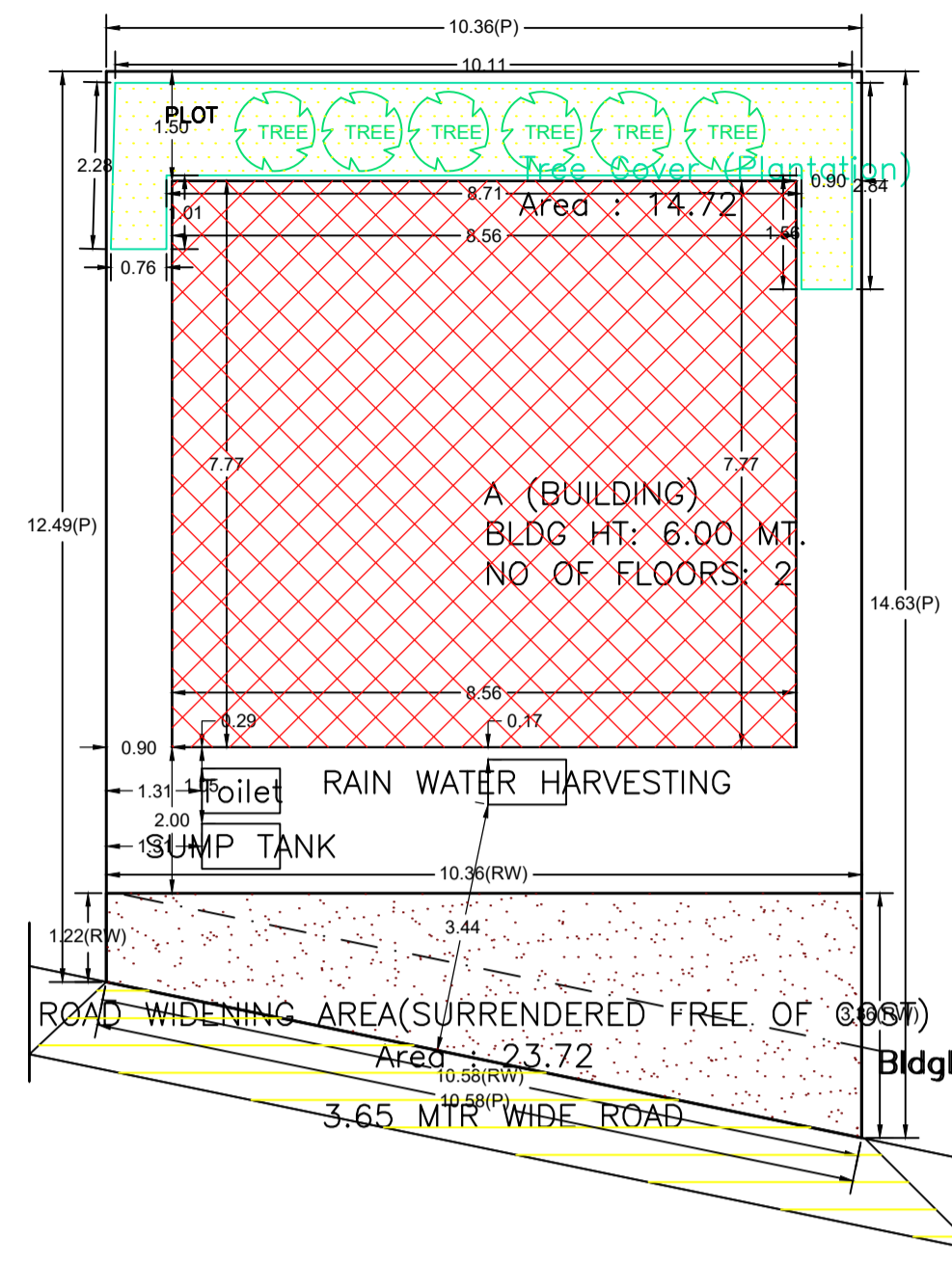
SITE PLAN
