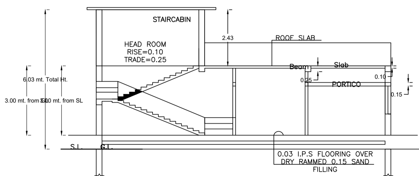
SECTION ON-XX
