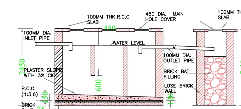
SEPTIC TANK DETAIL
