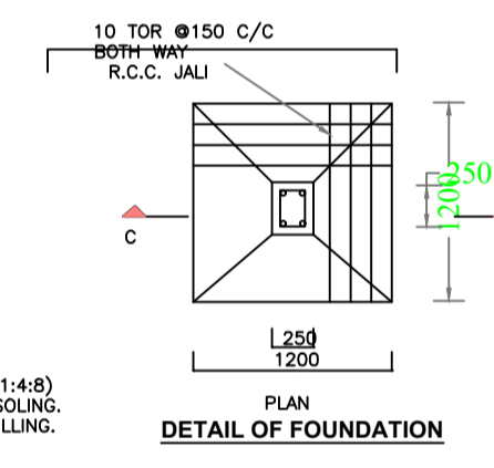
DETAIL OF FOUNDATION
