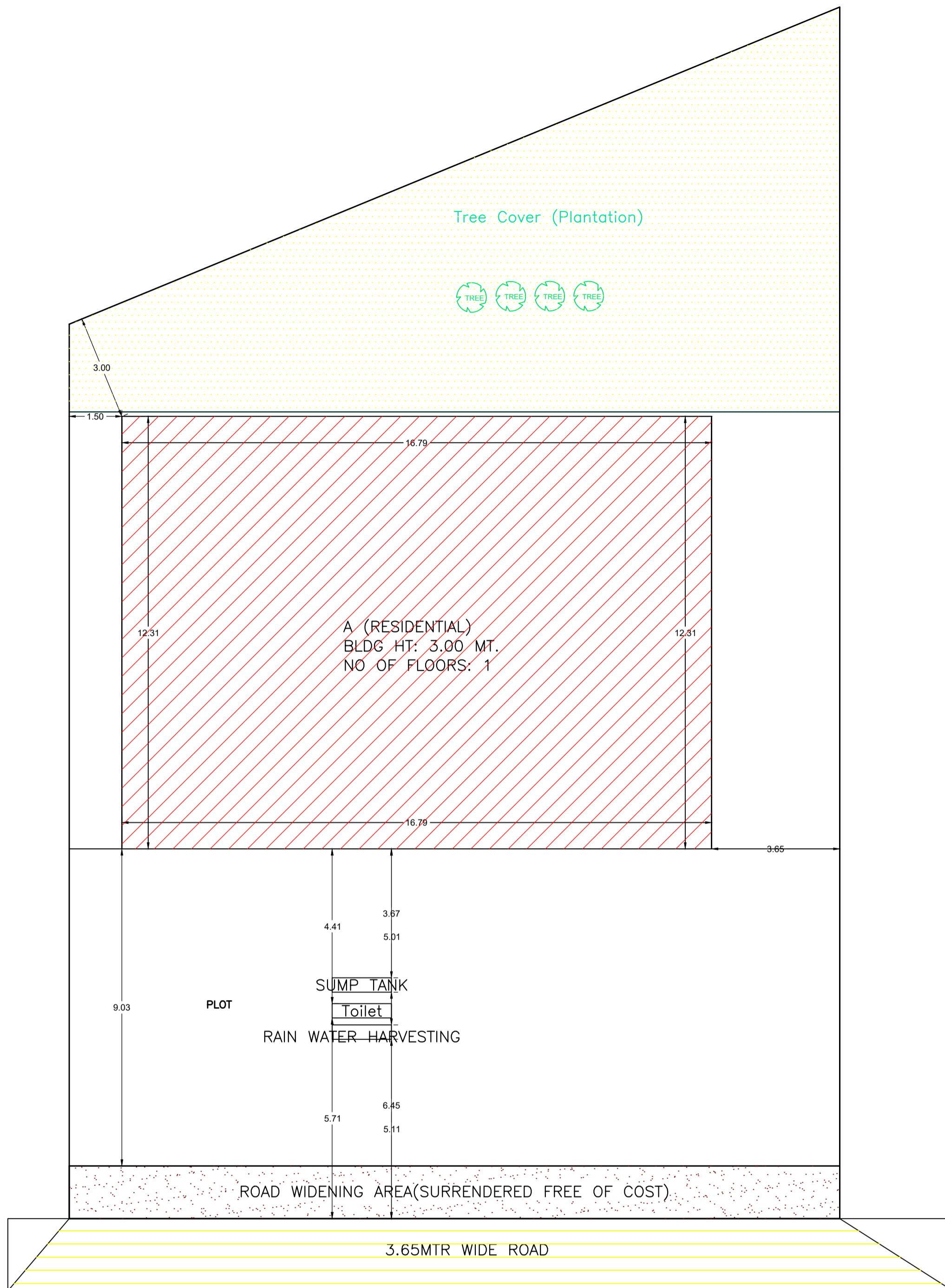
SITE PLAN
