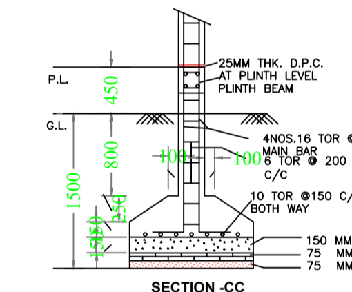
STRUCTURAL DETAIL
