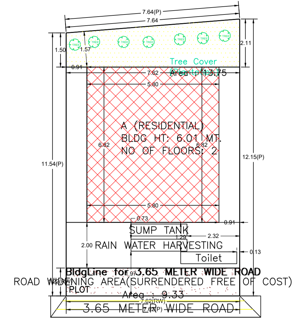
SITE PLAN
