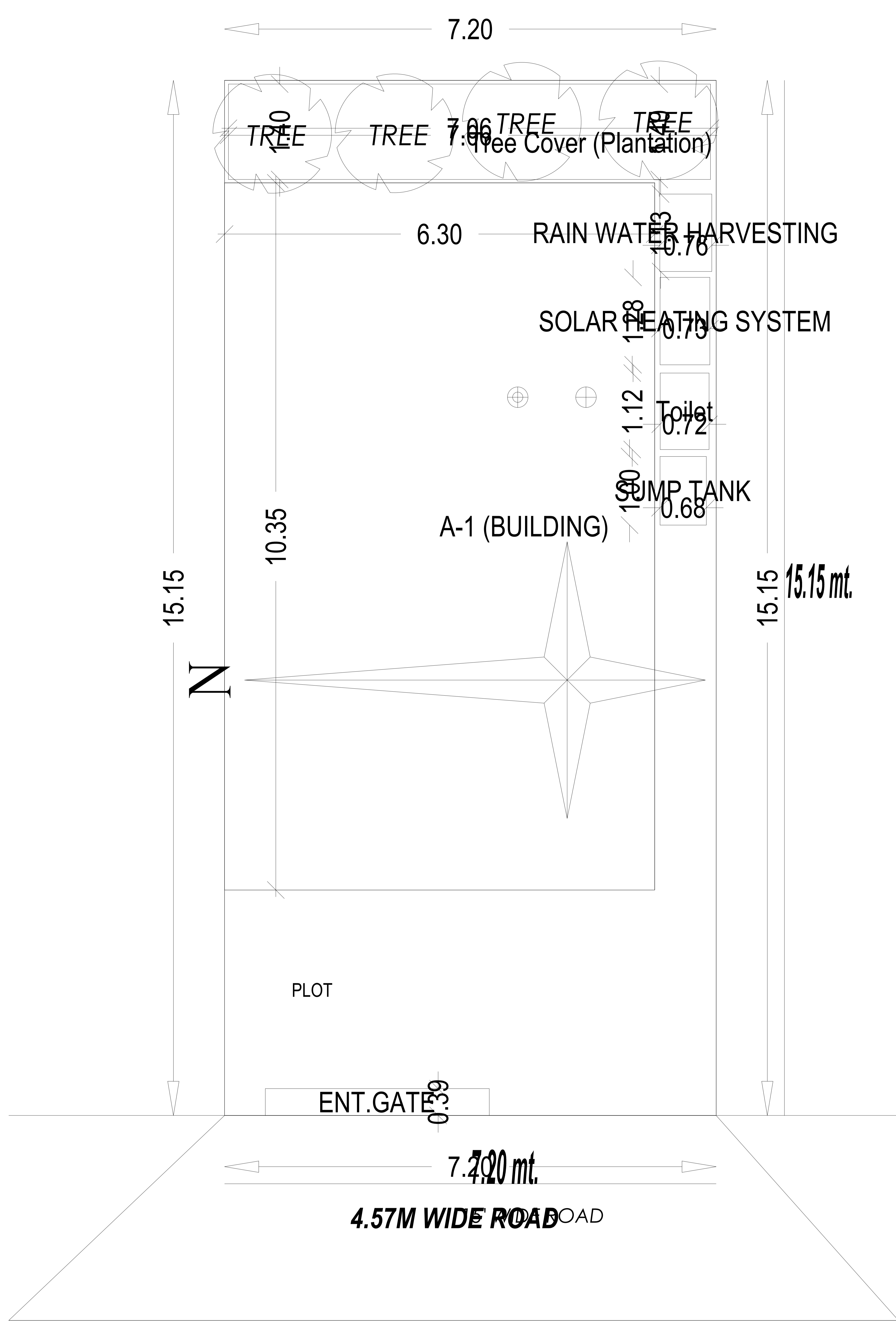
SITE PLAN
