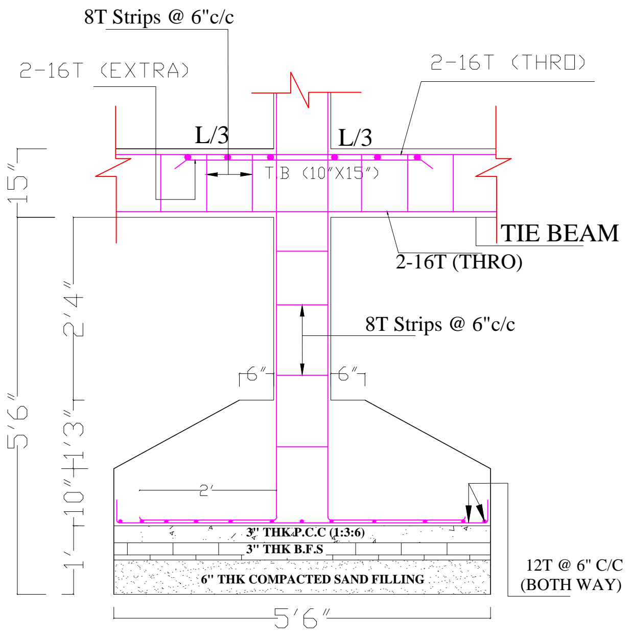
SECTION - B-B
