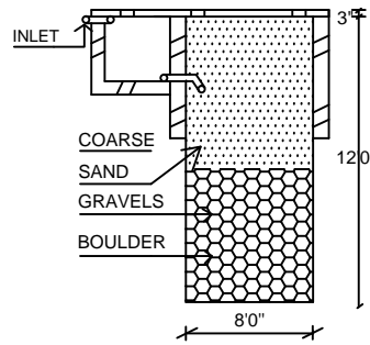
Rain Water Storage Tank Detail RAIN WATER HARVESTING SCHEME
