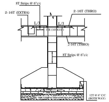
Structure Detail
