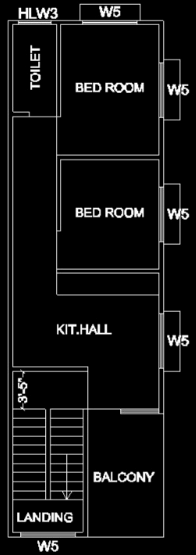
2ND FLOOR PLAN
