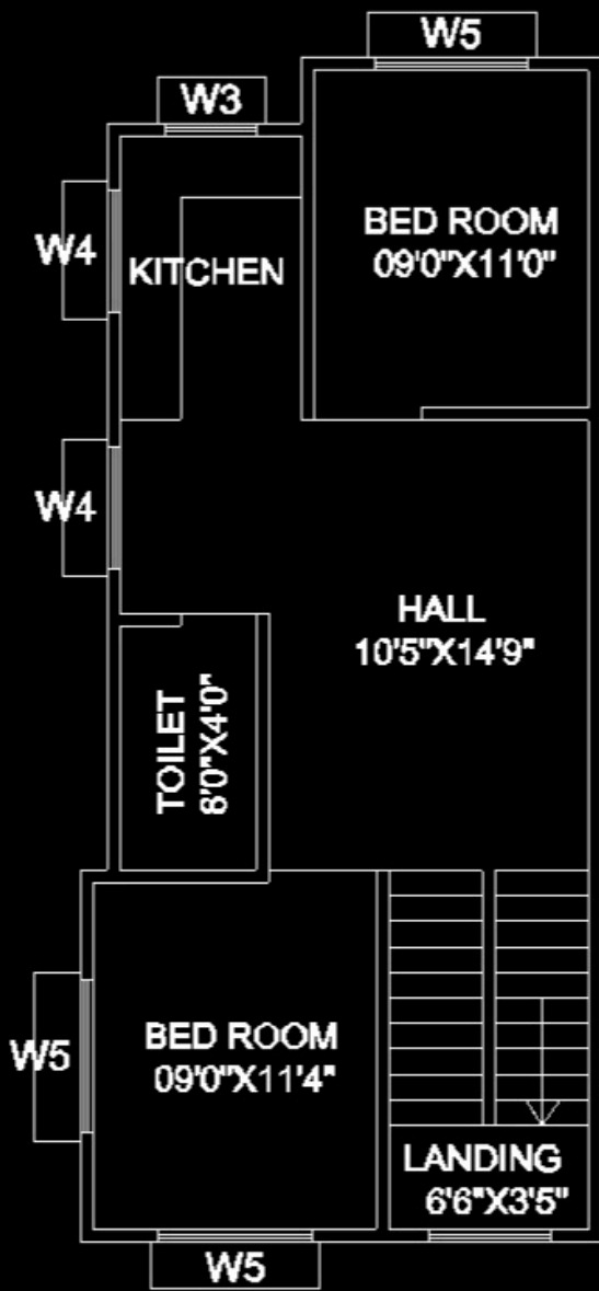
GROUND FLOOR PLAN BUILT UP AREA= 728.00 SQ.FT
