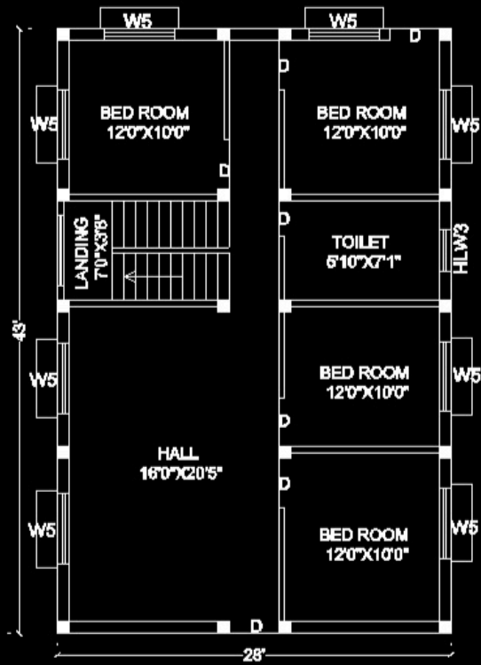
GROUND FLOOR PLAN BUILT UP AREA.1200.00 SQ.FT
