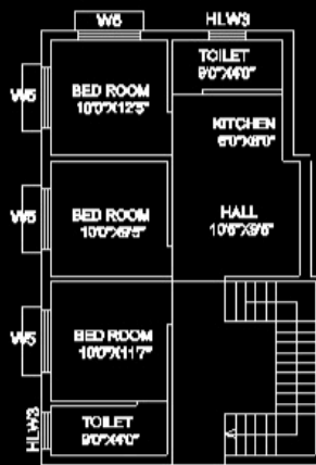
1ST FLOOR PLAN BUILT UP AREA= 559.56 SQ.FT
