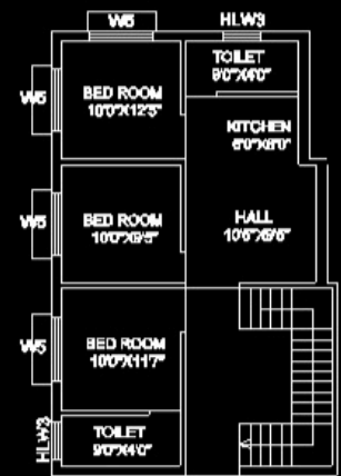
2ND FLOOR PLAN BUILT UP AREA= 559.56 SQ.FT
