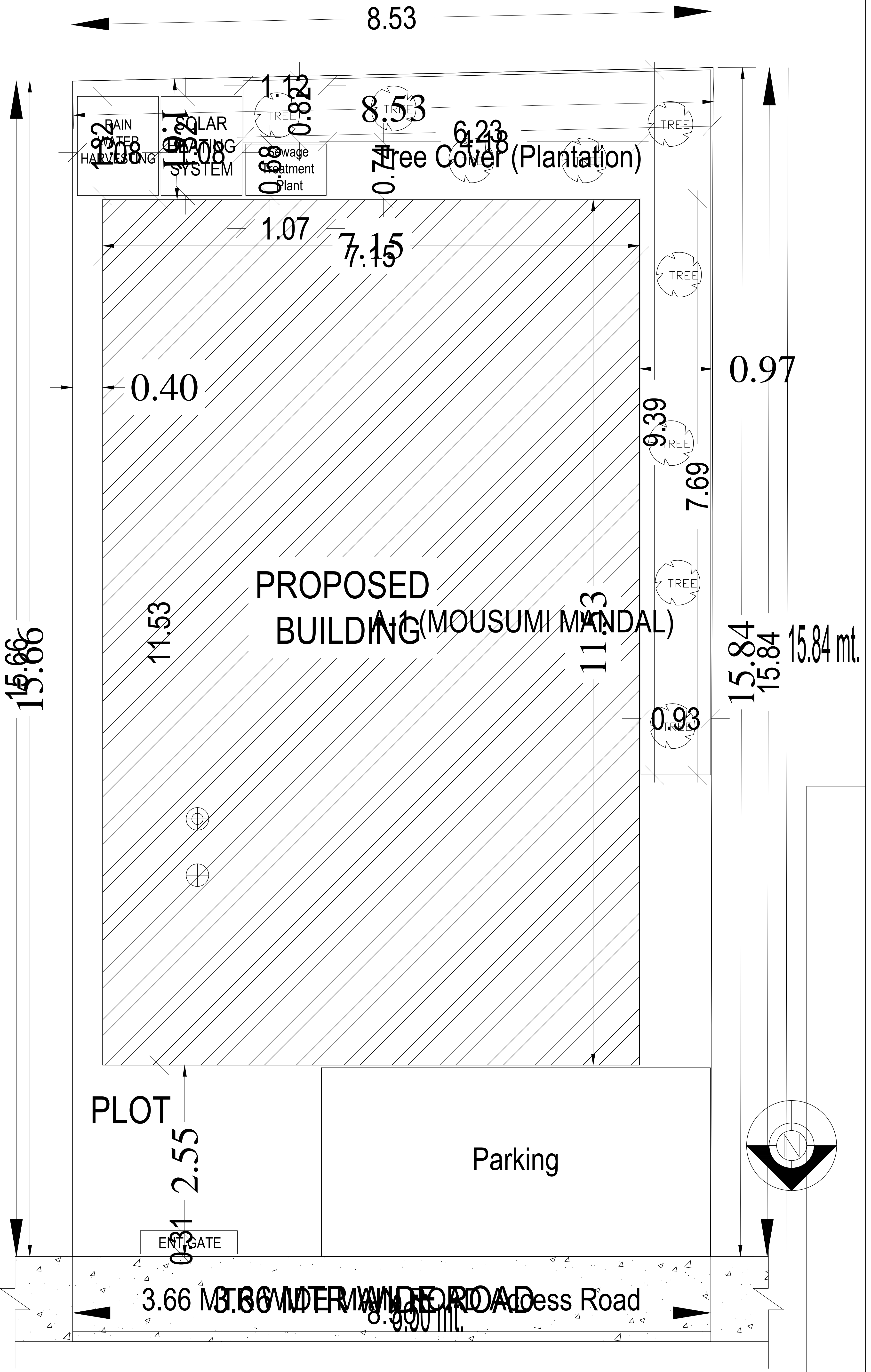
SITE PLAN
