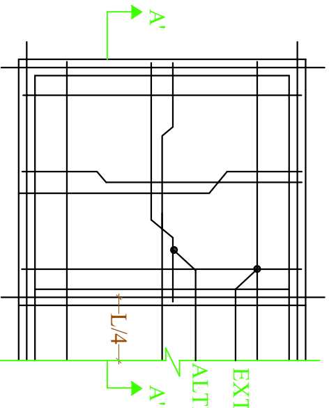
TYPICAL REINFORCEMENT DETAIL
