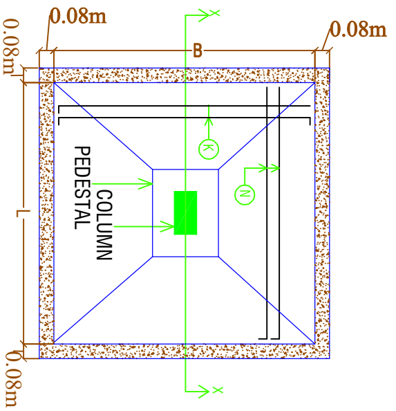
PLAN OF ISOLATED FOOTING
