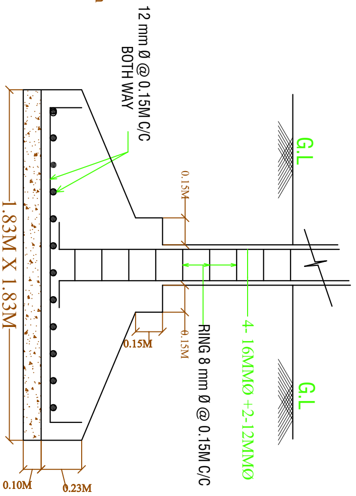
SECTION OF FOOTING .
