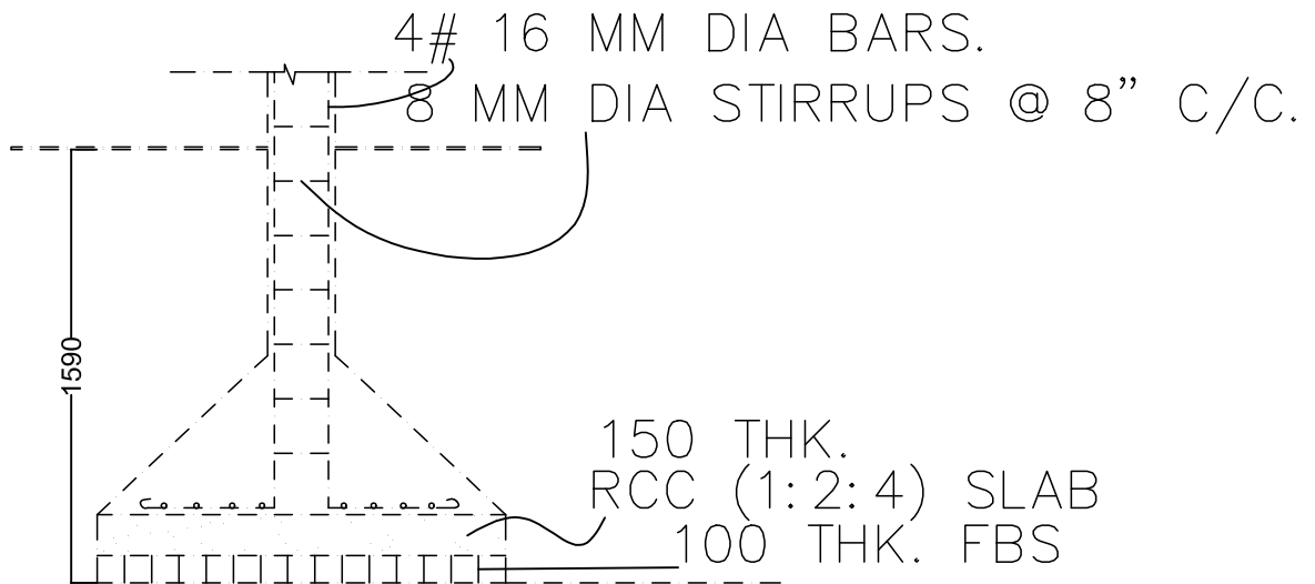
SECTION FOUNDATION DETAILS (ISOLATED R.C.C FOOTING)
