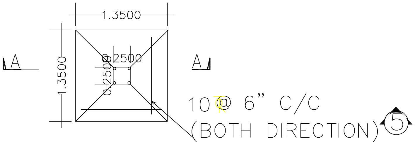
FOUNDATION PLAN OF COLUMN
