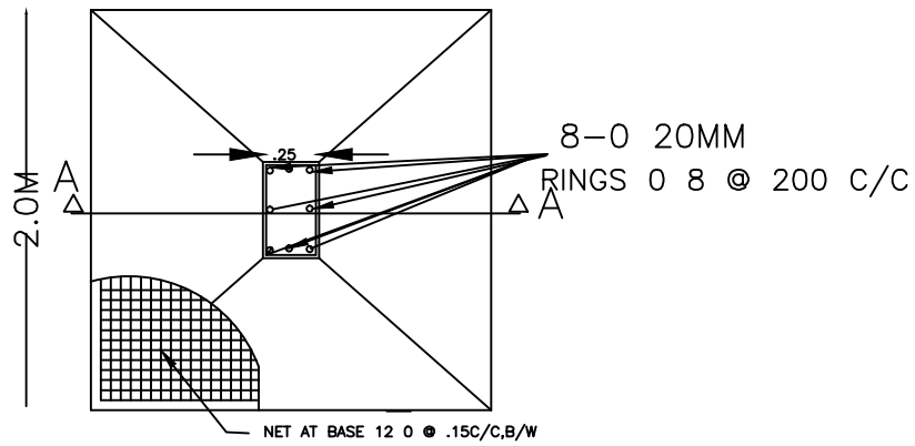
PLAN OF COLUMN FOUNDATION
