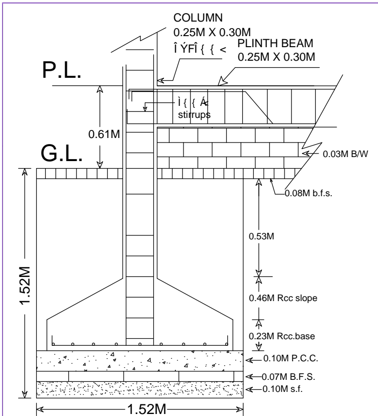
C/S OF EXSISTING FOOTING
