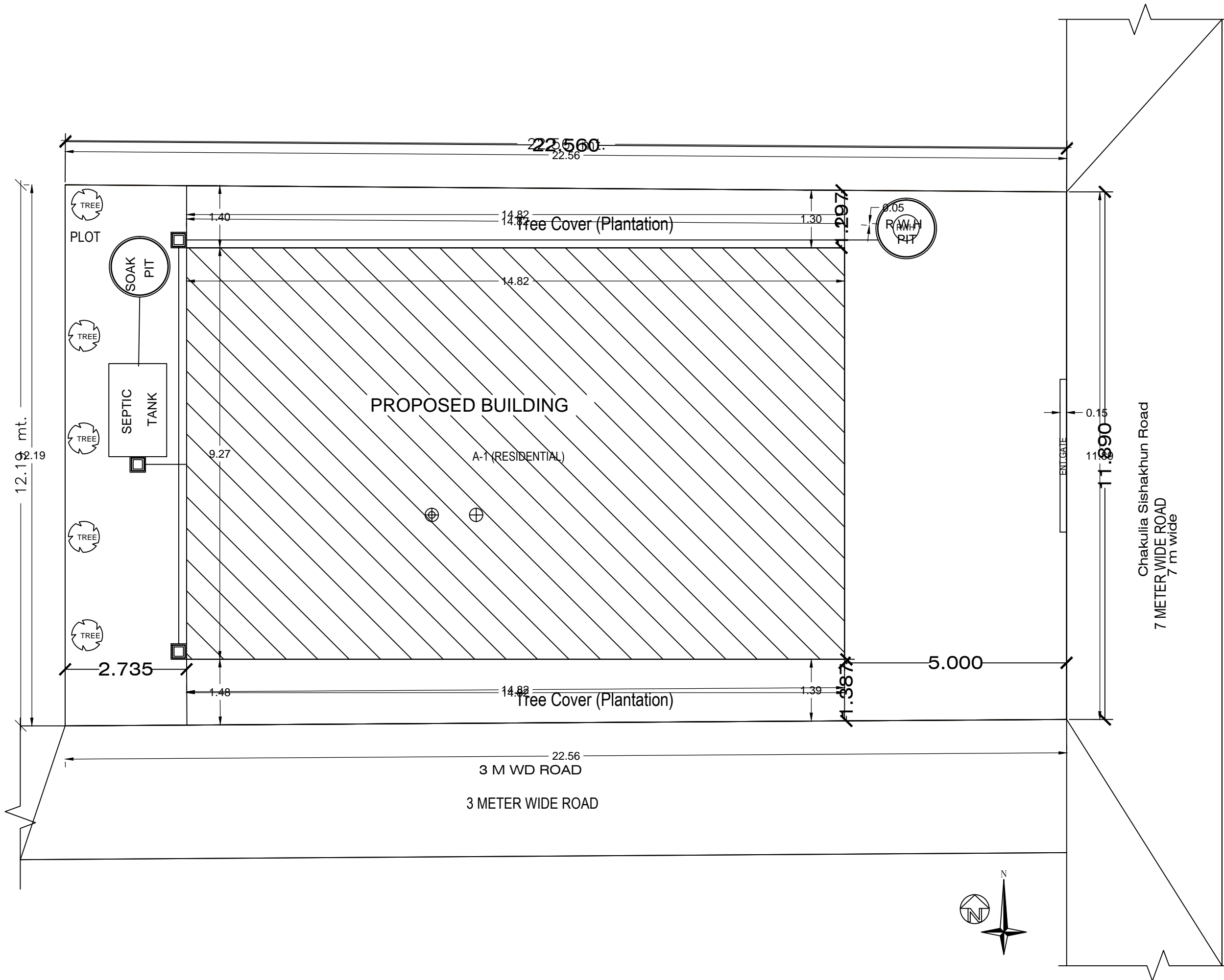
SITE PLAN
