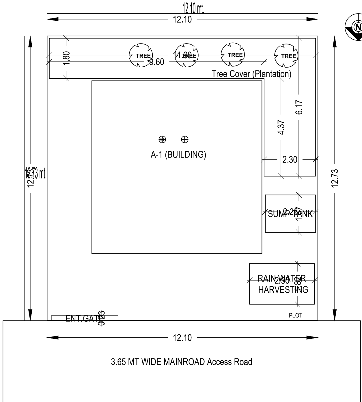
SITE PLAN
