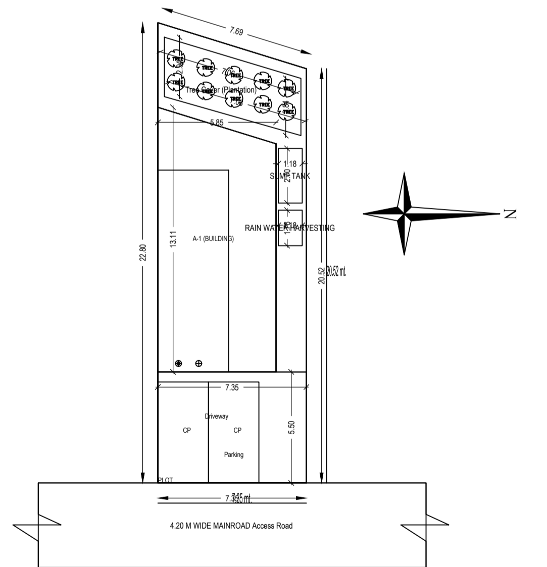
SITE PLAN
