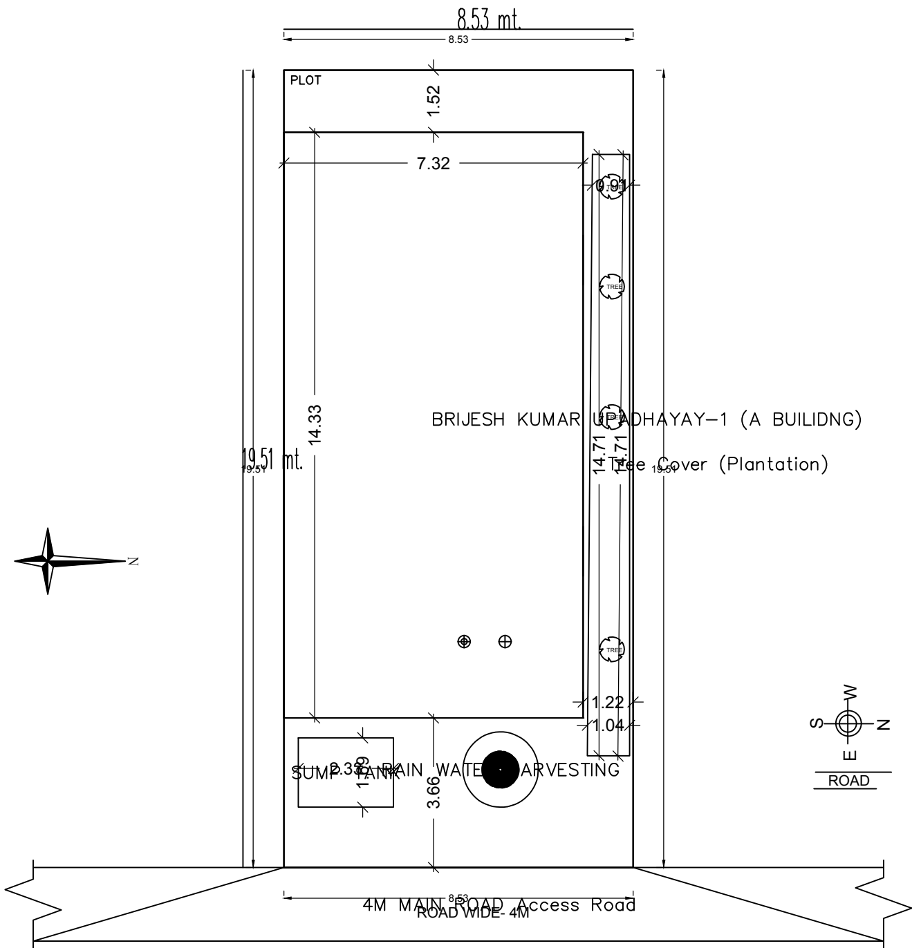
SITE PLAN
