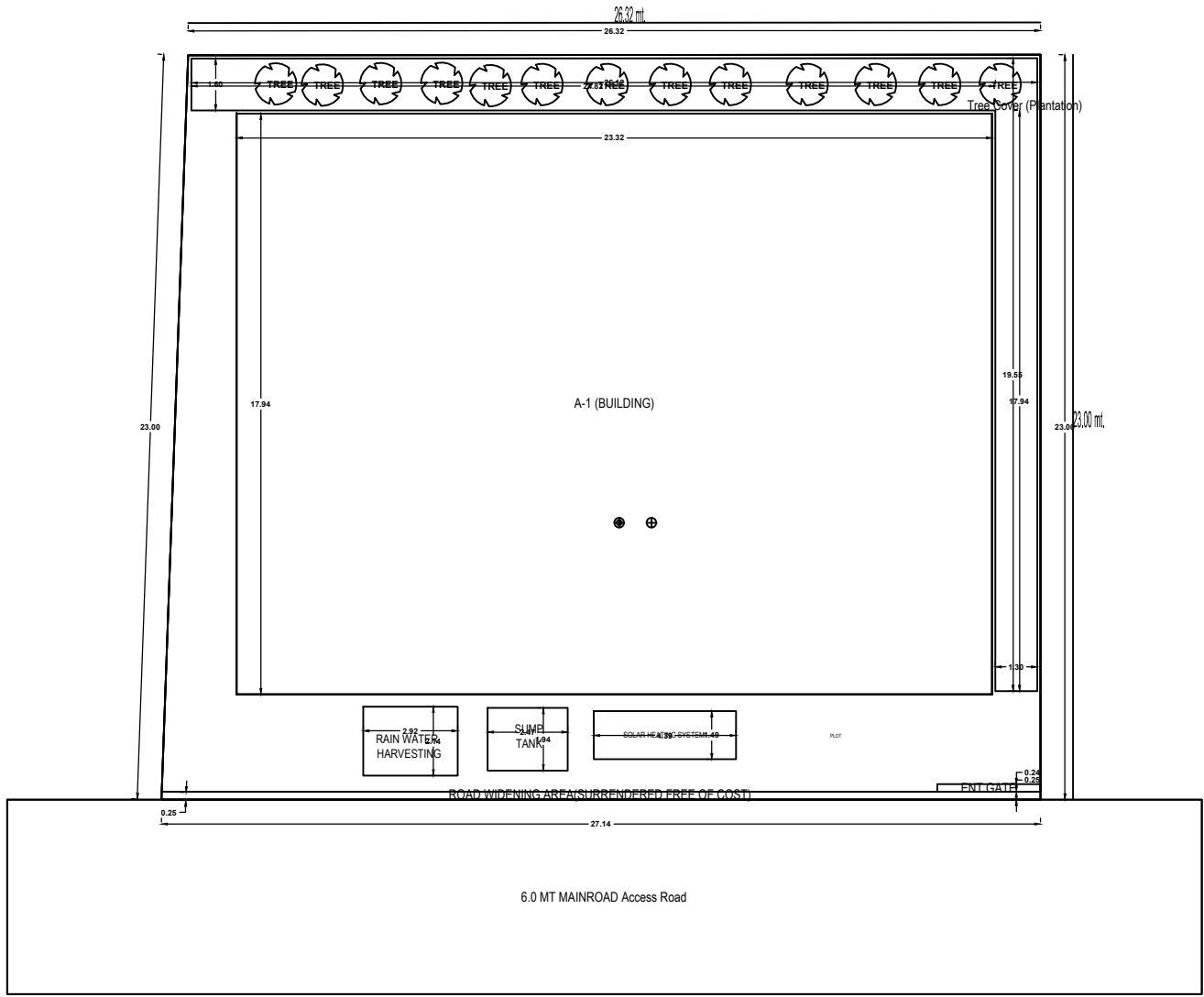
SITE PLAN
